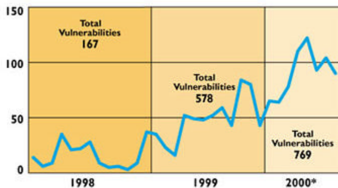
Figure 1: Bugtraq vulnerabilities by month from January 1998 to September 2000.
